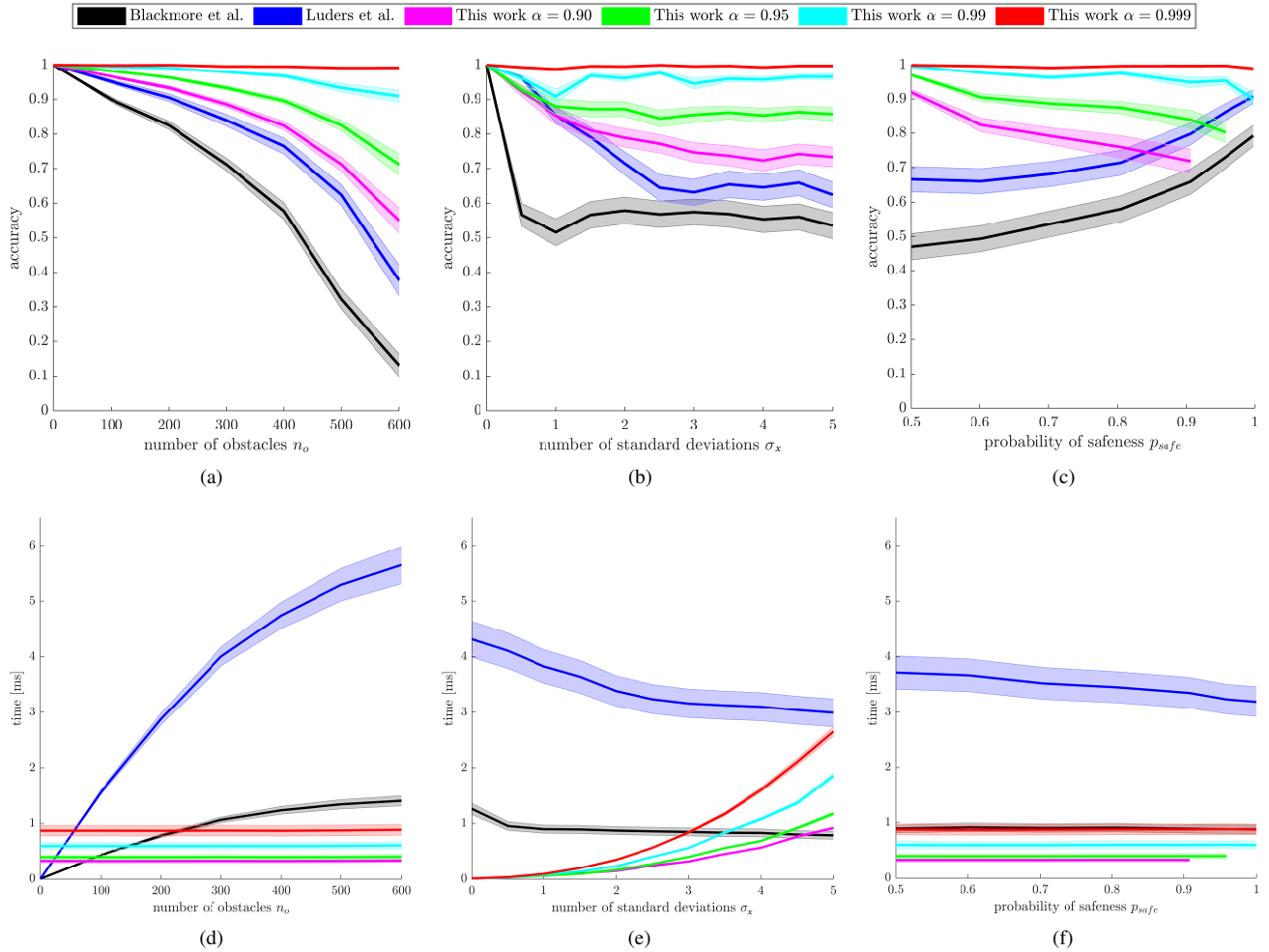
Fig. 14: Evaluation of the accuracy (first row) and performance (second row) of the chance constraints formulations [9, 46] and the proposed probabilistic collision checking method with \alpha = \{0.90, 0.95, 0.99, 0.999\} . The accuracy and performance metrics are represented subject to the number of obstacles n_o in the environment (first column), the state uncertainty \Sigma_x = \sigma_x^2 \mathbb{I}_{3 \times 3} (second column), and minimum safety probability bound p_{\text{safe}} (third column). The shadowed area corresponds to the variance of the metrics. In the interest of clarity, only one tenth of the variance is displayed.
