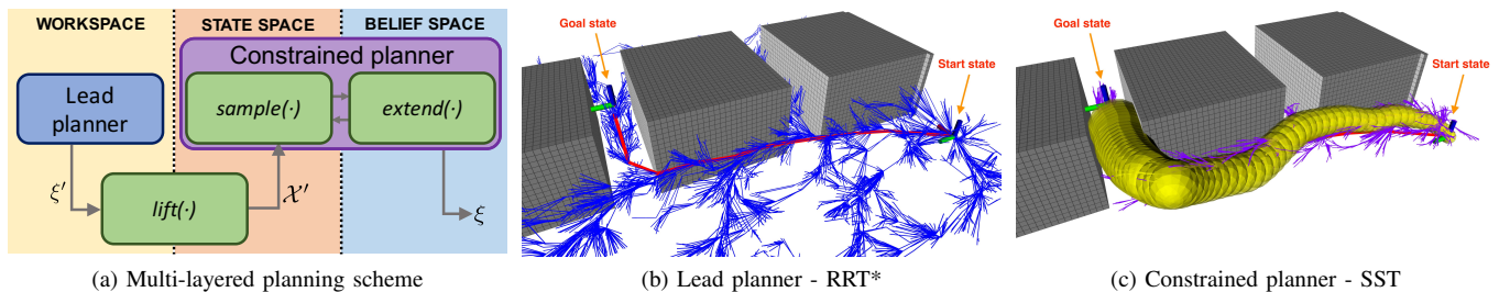
Fig. 3: Multi-layered motion planning framework: the lead planner shown in blue in (b) computes a geometric lead \xi' (red path) to guide the search space \mathcal{X}' of the constrained planner shown in magenta in (c). The resulting trajectory \xi with its uncertainty (yellow funnel) satisfies kinodynamic and probabilistic safety constraints.
