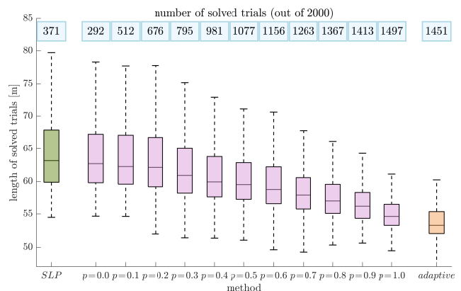
Fig. 12: Performance of (i) our precedent single-layered planning (SLP) scheme (green) and the newly proposed multi-layered scheme when considering (ii) a fixed lead with different bias p (magenta, with best radius as found in Figure 11), or (iii) an adaptive lead as defined in Figure 13 (orange).
