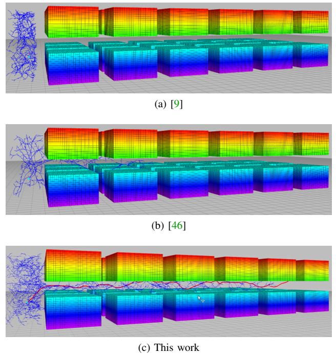
Fig. 15: Effect of conservatism in the workspace. The over-conservatism of chance constraints formulations [9, 46] impedes finding a solution. Our probabilistic collision checking with a fixed conservatism \alpha succeeds on finding a trajectory which transverses the environment with a total of 36 obstacles.
