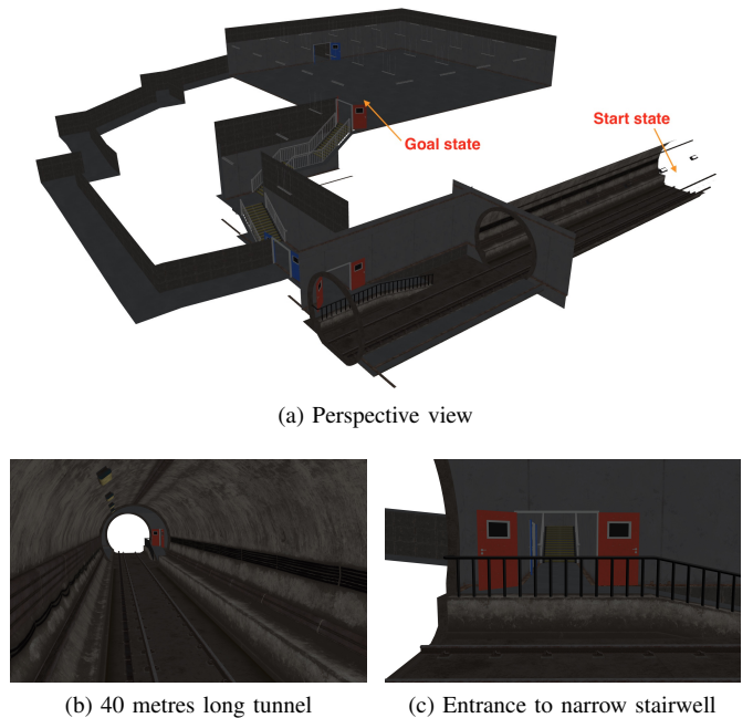
Fig. 16: Urban Stairwell scenario of the DARPA Subterranean Challenge 2019. (a) Start-to-goal query which requires traversing (b) a 40 metres long tunnel and (c) a narrow 25 metres long stairwell. Planning through the stairwell is particularly challenging due to the accumulated localisation uncertainty.
