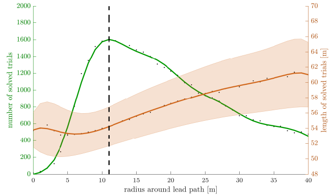
Fig. 11: Performance of the multi-layer planning scheme with a rigid- \mathcal{X}' , i.e., fixed radius around the geometric lead path.
