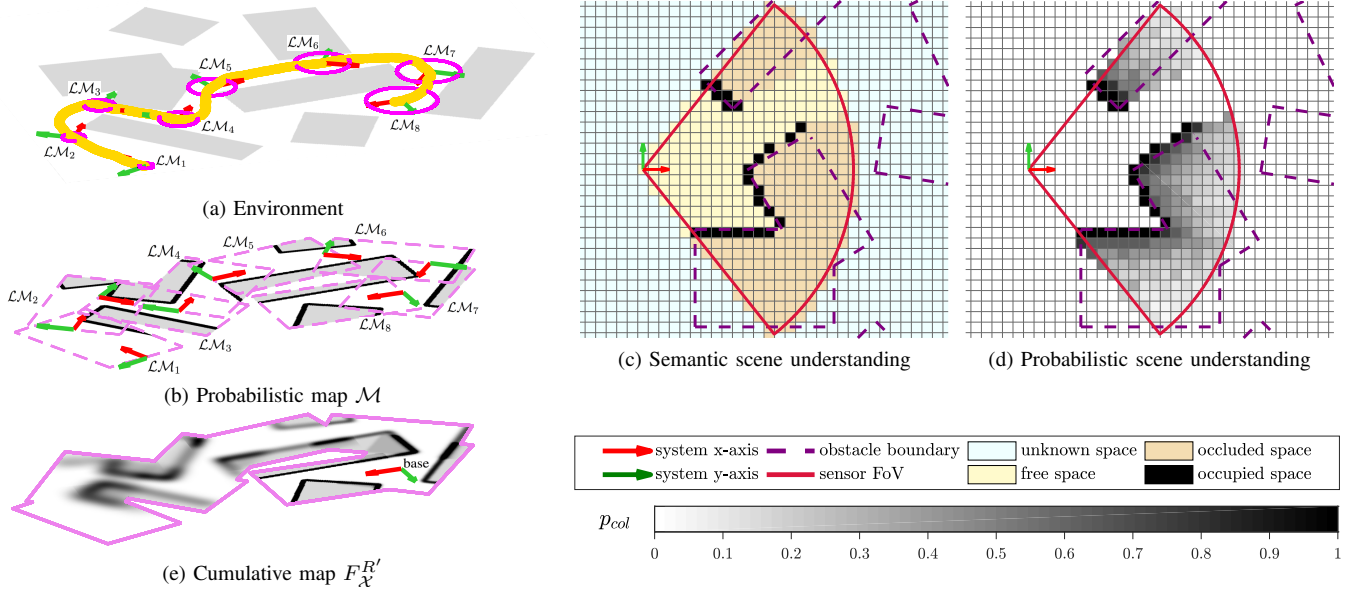
Fig. 2: Online mapping of the environment suitable for motion planning under uncertainty. (a) As the robot navigates through an unknown environment, (b) it builds a probabilistic map \mathcal{M} which represents the surroundings as a set of local maps. Each local map is uncertain (magenta ellipses in (a)) with respect to the global frame. (c-d) Each local map is encoded as an occupancy grid map, which is build from a set of sequential sensors scans over a finite horizon time. (e) All local maps are fused into a cumulative map representation F_{\mathcal{X}}^{R'} taking into account the relative uncertainty of each local map with respect to the predicted planning frame R' . Note: our mapping suits 3D scenes too; illustrations in 2D for visualisation purposes only.
