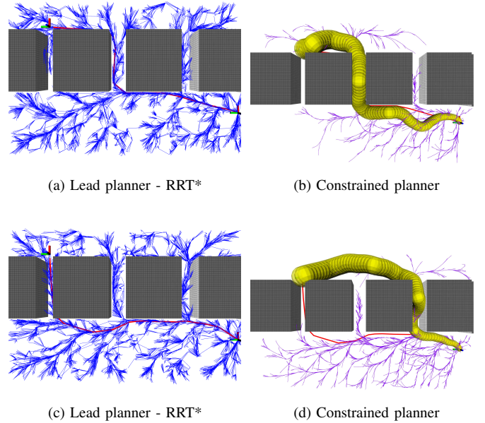
Fig. 4: Probabilistic completeness of the proposed multi-layered planning scheme with adaptive lead, which (a-b) promotes finding the final solution in the neighbourhood of the asymptotically optimal lead \xi' (red), while it (c-d) preserves completeness guarantees even when the lead \xi' transverses a corridor which does not offer a probabilistic safe passage.
