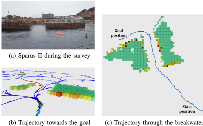
Fig. 9: Sparus II AUV guided by the proposed uncertainty-based framework to solve a start-to-goal query in an undiscovered environment.
